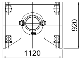
PUMP-TROLLEY
